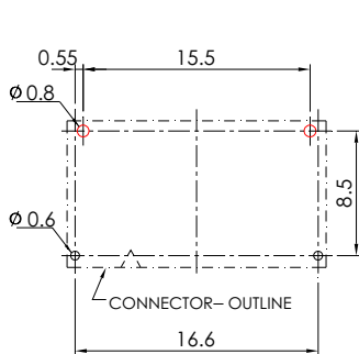
P. C. BOARD LAYOUT DIP Application (TYPE-E)
