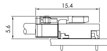
ASSEMBLY (DIP)
