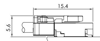
ASSEMBLY (SMT)
