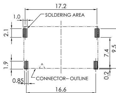
P. C. BOARD LAYOUT SMT Application (TYPE-B)
