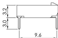
DIP Header
