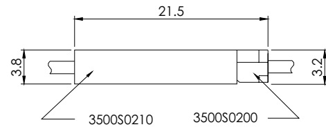
Assembly Layout
