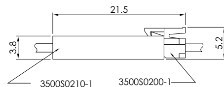
Assembly Layout
